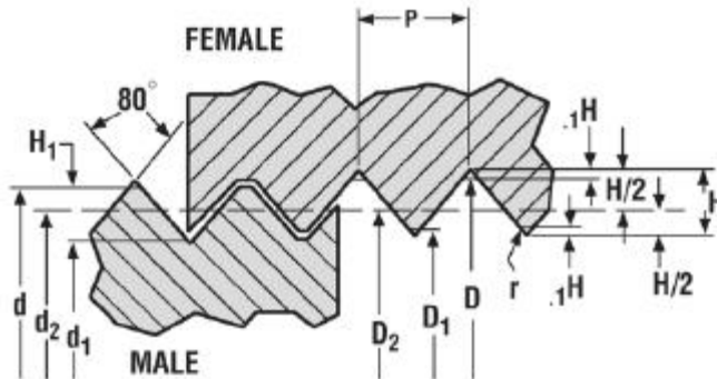
Machined Steel Pipe Thread-Limits (mm)
